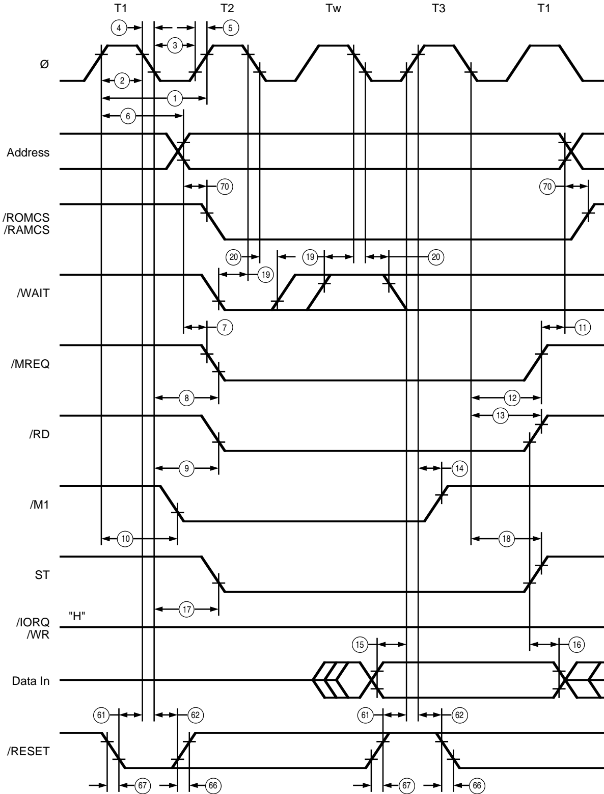
Figure 60a. Opcode Fetch Cycle
